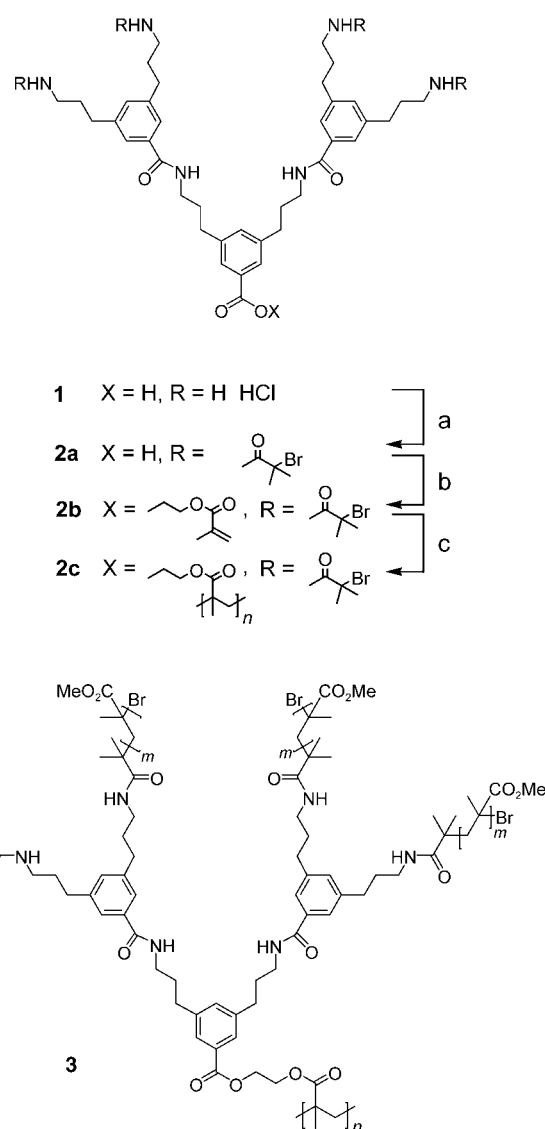
Scheme 1. Reagents and conditions: a) 1 , 2,5-dioxopyrrolidin-1-yl 2-bromoisobutyrate, TEA, CH 2 Cl 2 , MeOH, –30 °C, 15 h (86 %); b) 2a , DCC, HEMA, DMAP, CH 2 Cl 2 , RT, 15 h (68 %); c) 2b , DCM, 55 °C, 8 h (85 %). TEA = triethylamine, DCC = N,N' -dicyclohexylcarbodiimide, HEMA = hydroxyethylmethacrylic acid, DMAP = 4-dimethylaminopyridine.
